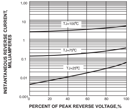
FIG. 4-TYPICAL REVERSE CHARACTERISTICS
